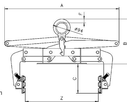
Concrete grab with large jaw capacity
